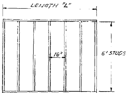
END WALL AND ENTRYWAY PANELS ALL STUDS 2"x4" X 6' HIGH ALL STUD PLATES 2"x4" 12 PANELS REQUIRED
